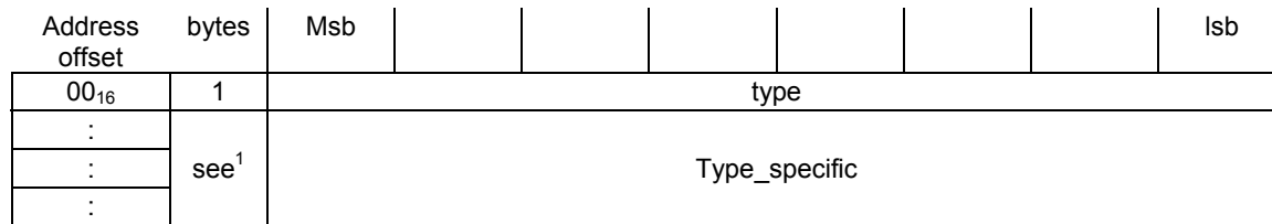
Figure 9.26 – List_descriptor_specifier
