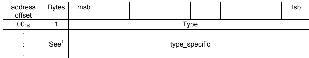
Figure 9.25 – Entry_descriptor_specifier
